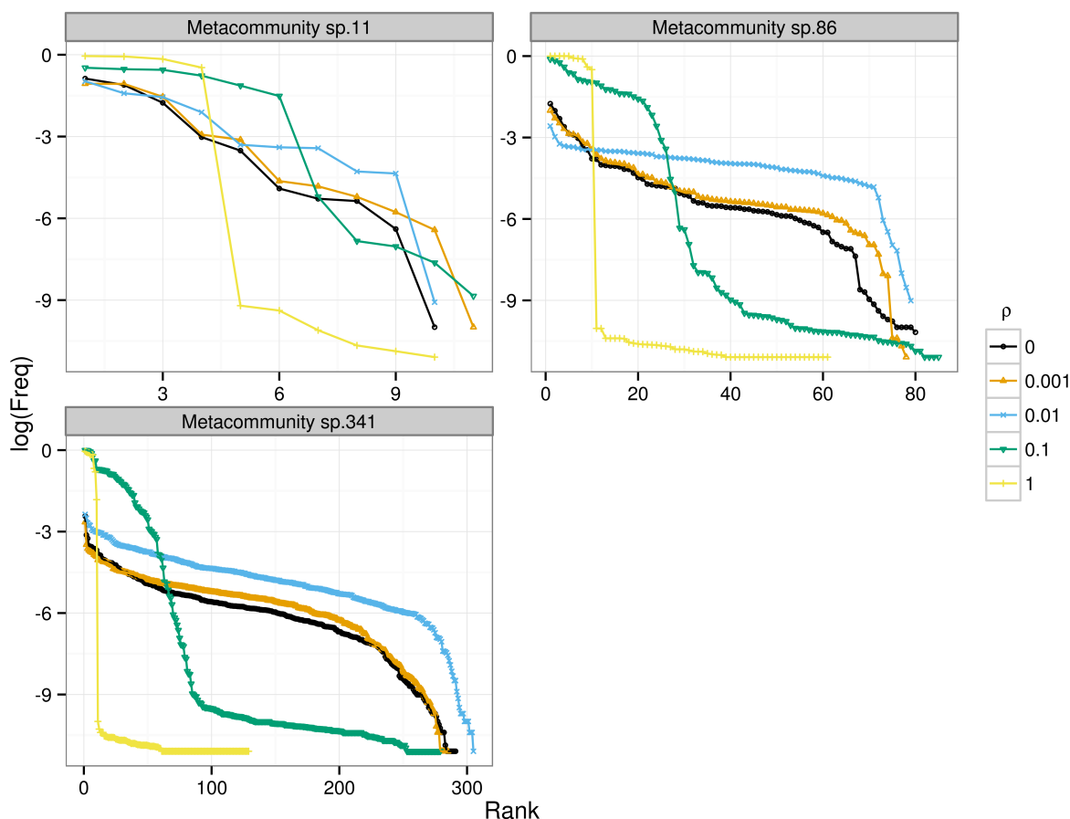
Figure 5: Rank abundance diagrams of communities patterns generated with a spatial neutral/hierarchical model with different number of species in the metacommunity (labeled in each subfigure). \rho is the parameter that determines the degree of neutrality. When this parameter is 0 the model is completely neutral and there is no competitive replacement of species. When \rho is 1 competitive superior species always replaces inferior ones and the model is completely hierarchical. The simulations use a metacommunity with a logseries abundance distribution with 11, 86 and 341 species and a simulation grid side=256, the other parameters used were MortalityRate=0.2, DispersalDistance=0.4 (2.5 grid units), ColonizationRate=0.001. The ranks were calculated with averages of species densities over 50 simulations.
