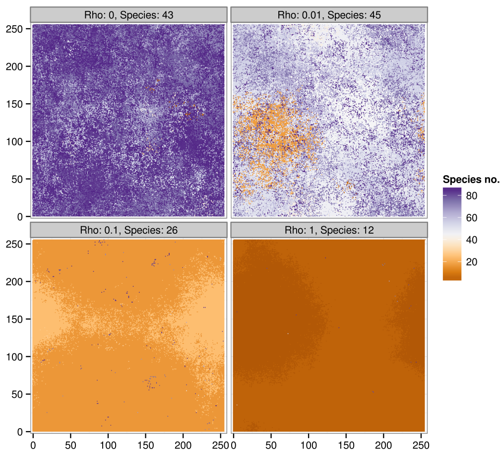
Figure 4: Spatial patterns generated with a spatial neutral/hierarchical model. Rho is the parameter that determines the degree of neutrality. When this parameter is 0 the model is completely neutral and there is no competitive replacement of species. When \rho is 1 competitive superior species always replaces inferior ones and the model is completely hierarchical. Species is the number of species actually present plot. The simulations use a metacommunity with a logseries abundance distribution with 86 species and a simulation grid side=256.
