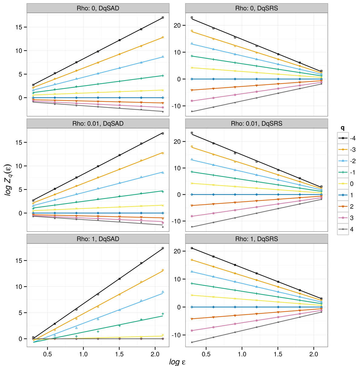
Figure 6: Linear fit of Z_q(\epsilon) to estimate generalized dimensions ( D_q ) from spatial patterns generated with a neutral/hierarchical model. \rho is the parameter that determines the degree of neutrality. When this parameter is 0 the model is completely neutral and there is no competitive replacement of species. When \rho is 1 competitive superior species always replaces inferior ones and the model is completely hierarchical. \text{Species} is the number of species actually present plot. The simulations use a metacommunity with a logseries abundance distribution with 86 species and a simulation grid side=256 sites.
