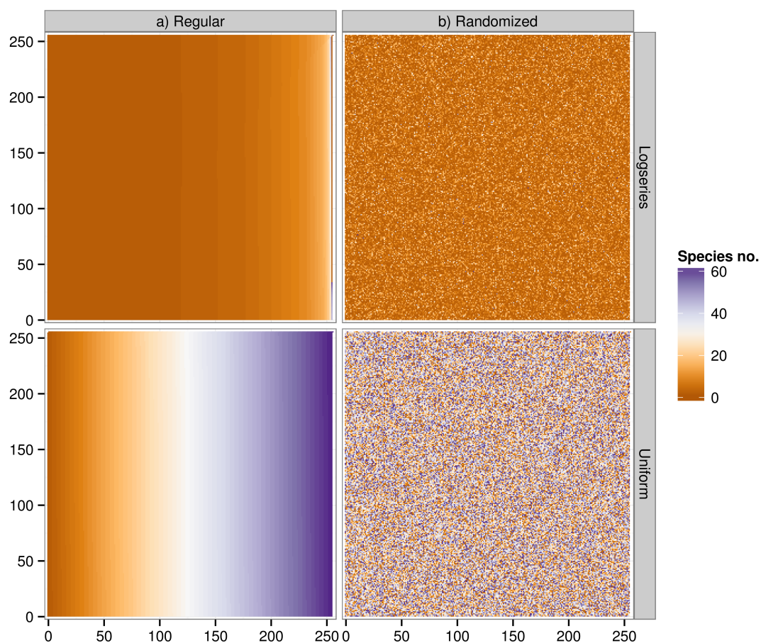
Figure 1: Spatial patterns generated with logseries and uniform species abundance distribution (all species have the same density) with 64 species and a grid with side=256. a) Regular: species are distributed in vertical bands. b) Randomized: the position of species are distributed at random in space.
