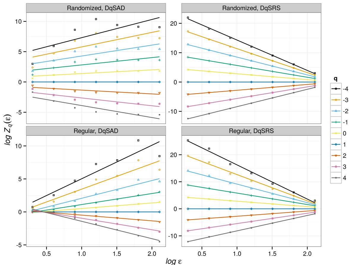
Figure 3: Linear fit of Z_q(\epsilon) to estimate generalized dimensions ( D_q ) from simple species spatial patterns with 64 species and a uniform abundance distribution. The spatial grid has a side=256 sites and two different spatial patterns: Regular, a regular spatial pattern with species distributed in vertical bands of equal width. Randomized, the positions of species in the grid are randomized. Two kinds of generalized dimension were estimated: DqSRS corresponds the fit of D_q^{SRS} (see text) and DqSAD is the fit from the estimation of D_q^{SAD} (see text). Z_q(\epsilon) corresponds to the partition function calculated for a box with side \epsilon , q is the moment order.
