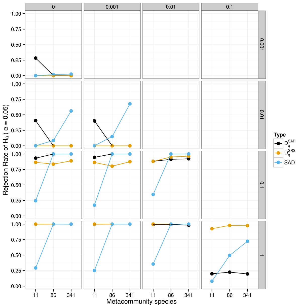
Figure 8: Power of the Anderson-Darling test for the hypothesis of differences between simulated neutral/hierarchical communities. The test uses generalized dimensions curves calculated from SAD ( D_q^{SAD} ), generalized dimensions calculated from the species rank surfaces ( D_q^{SRS} ) and the species abundance distributions (SAD). The compared communities differ only in parameter \rho (across panels) that determines the degree of neutrality/hierarchy. The number of comparisons to calculate the frequency is 2500 in all cases. Simulations use a metacommunity with a logseries abundance distribution with 11,86 and 341 species; a grid side of 256 sites, the other parameters are given in the main text.
